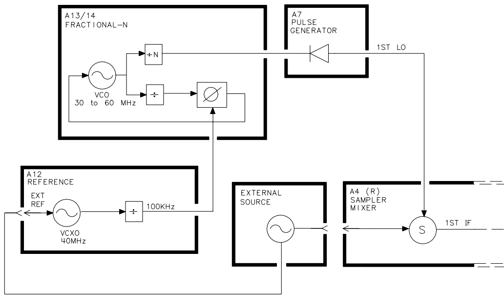
Figure 12-8 Tuned Receiver Mode
