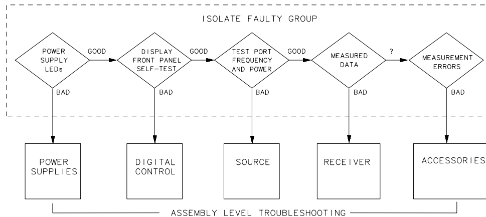
Figure 4-2 Troubleshooting Organization
