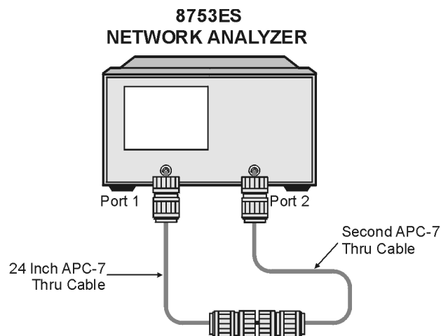
Figure 3-4 Second Connection for Insertion Loss Measurement
