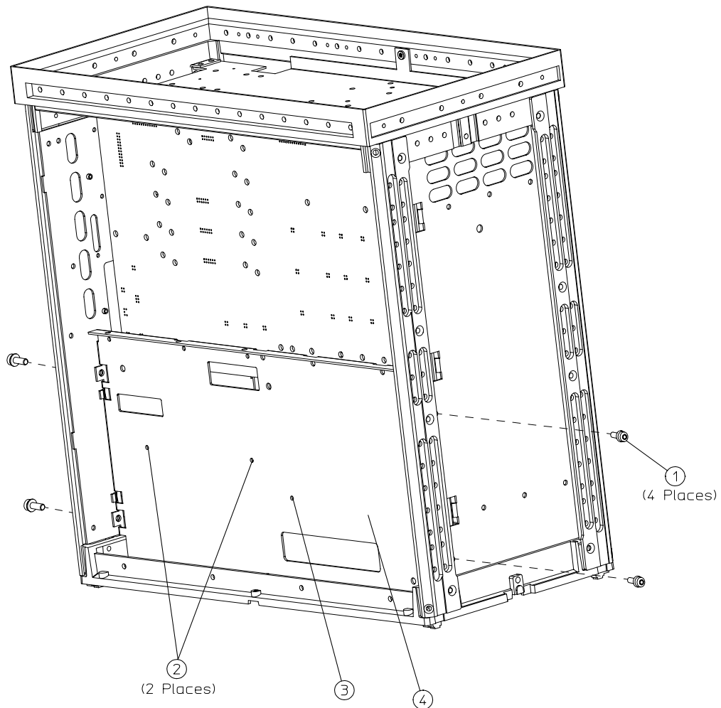
Figure 13-29 8753ET/ES: Hardware, Memory Deck
