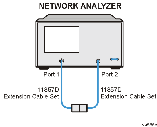
Figure 2-3 Transmission Calibration Setup
