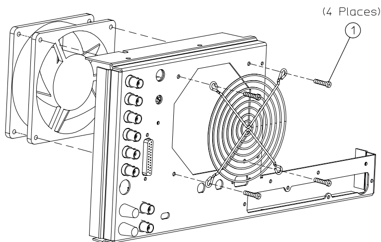
Figure 14-24 B1 Fan Assembly
