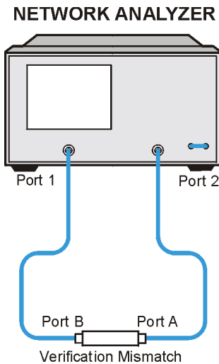
Figure 2-7 Mismatch Device Verification Setup 2
