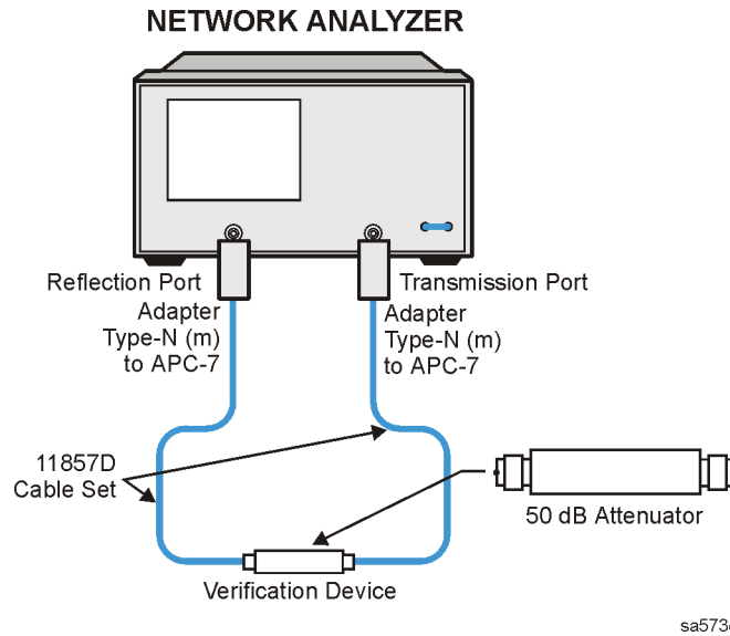
Figure 2-53 Connections for the 50 dB Verification Device
