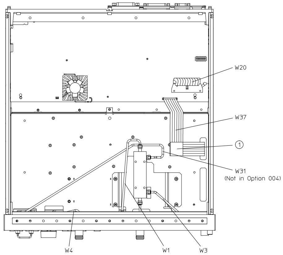
Figure 13-10 8753ET: Cables, Bottom
