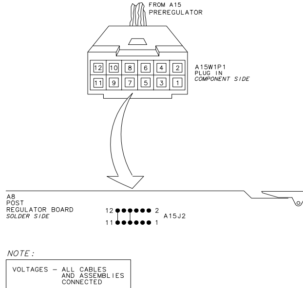
Figure 5-6 A15W1 Plug Detail
