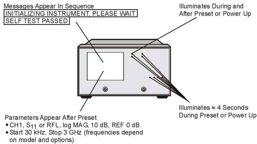
Figure 4-1 Preset Sequence
