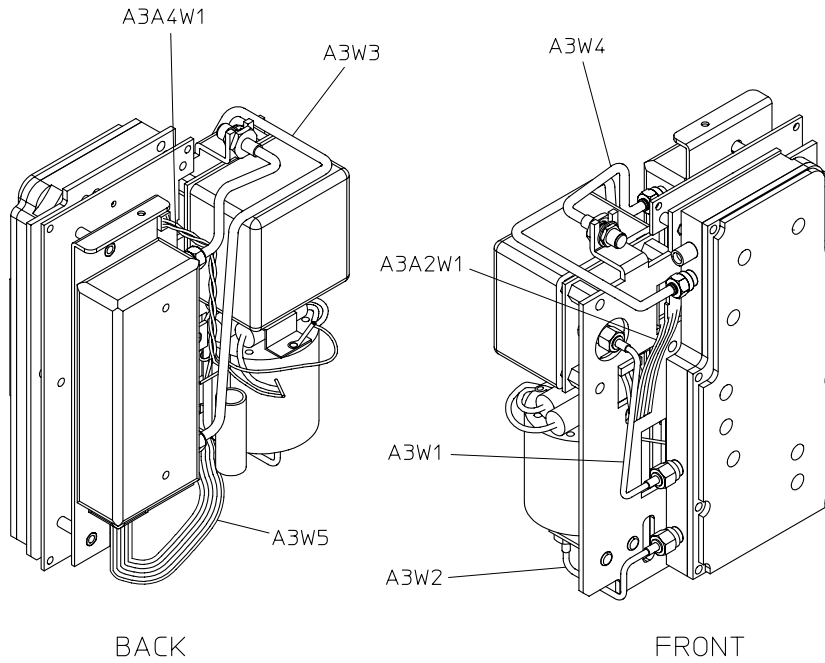
Figure 13-15 8753ES and 8753ET Option 004: Cables, Source
