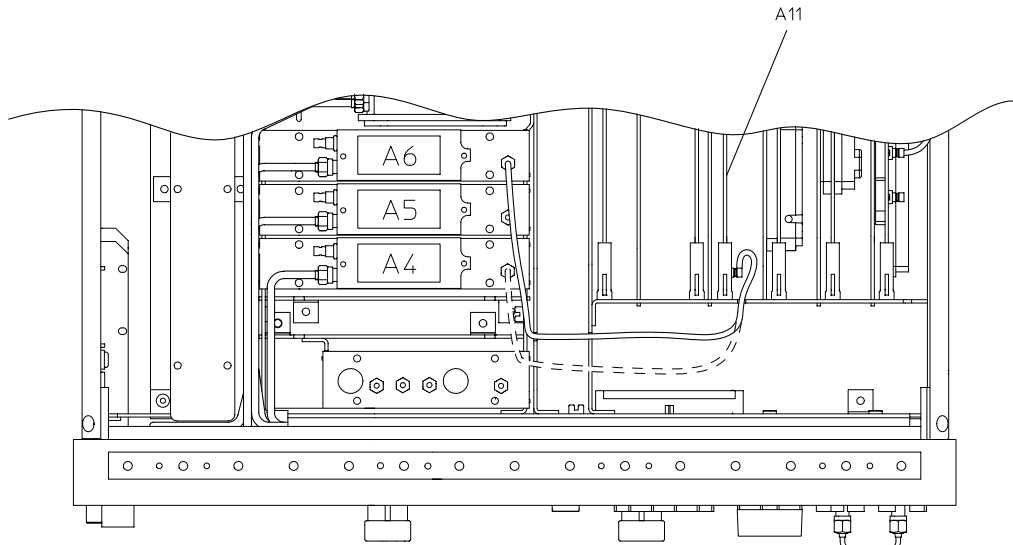
Figure 2-15 Connections for Substituting the R Sampler (A4)
