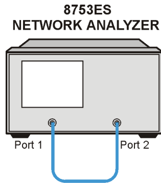
Figure 3-3 First Connections for Insertion Loss Measurement (8753ES)
