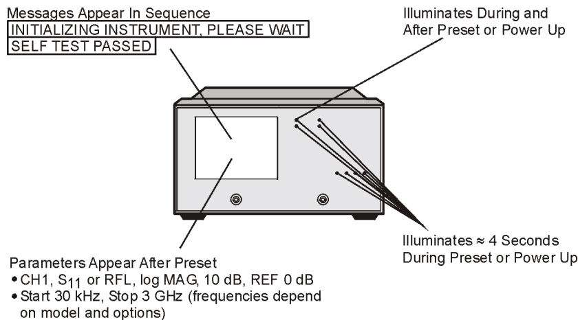
Figure 6-6 Preset Sequence
