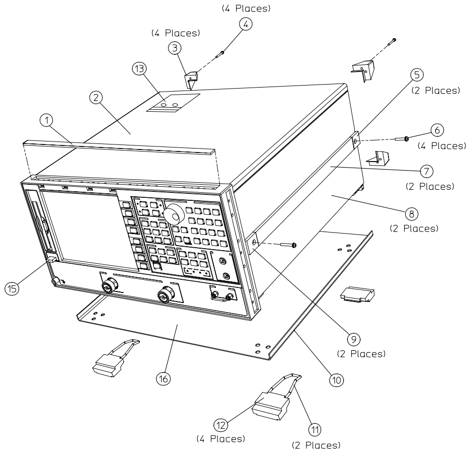
Figure 13-31 8753ET/ES: Chassis Parts, Outside
