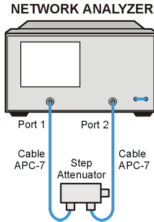
Figure 2-42 Test Port Phase Compression Test Setup
