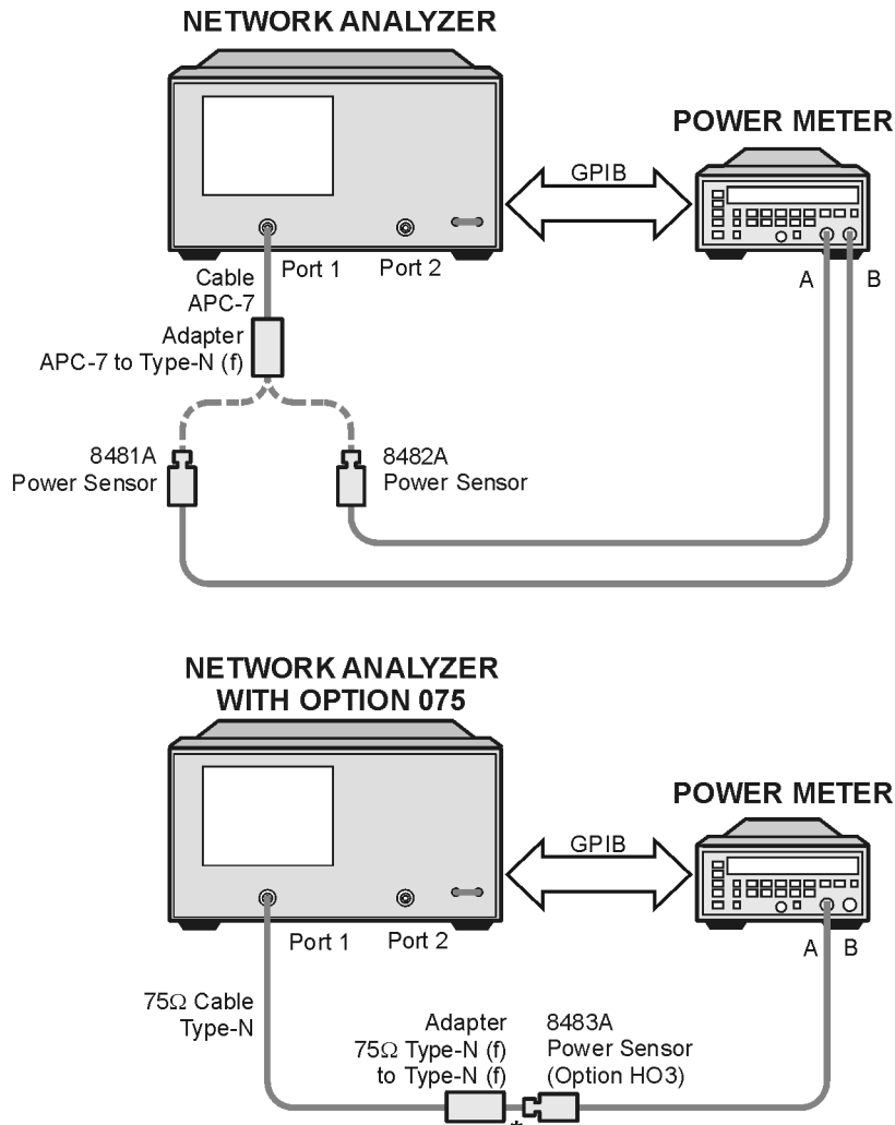
Figure 2-18 Setup for Power Meter Calibration on Test Port 1
