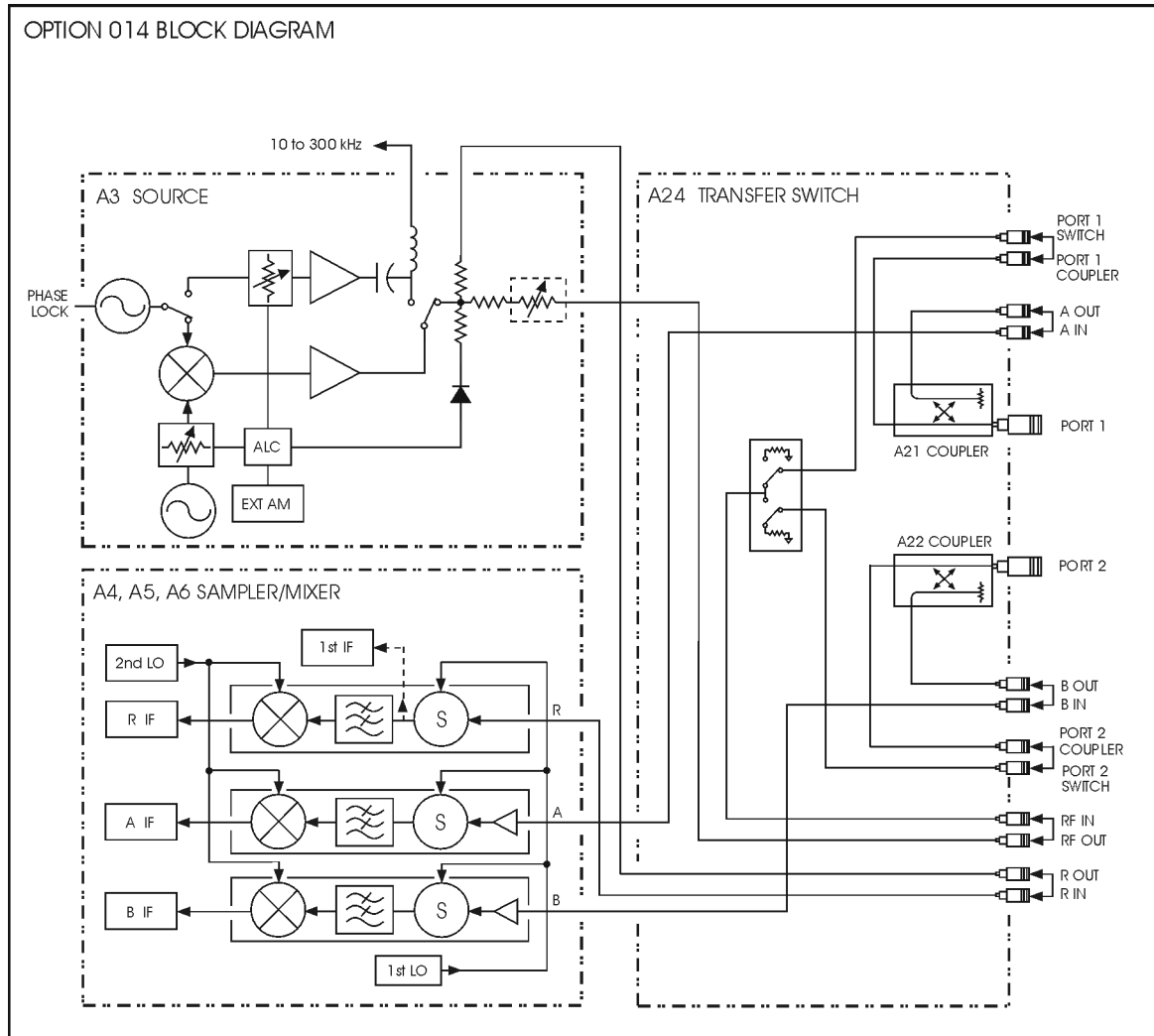
Figure 4-11 8753ES Option 014
