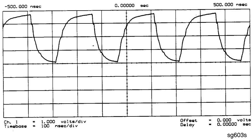
Figure 8-1 4 MHz REF Waveform
