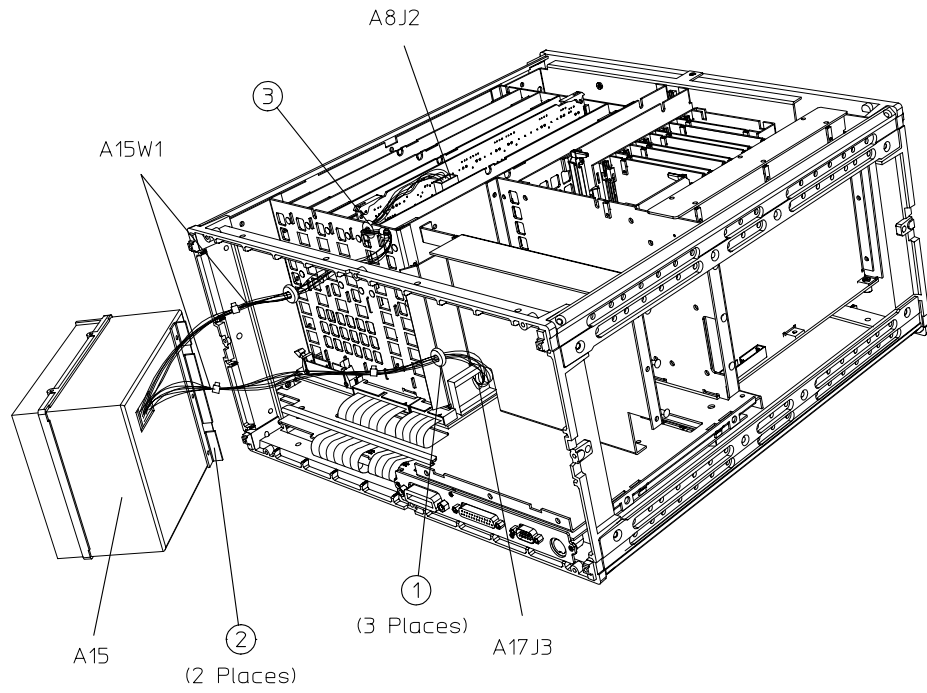
Figure 14-13 A15 Preregulator
