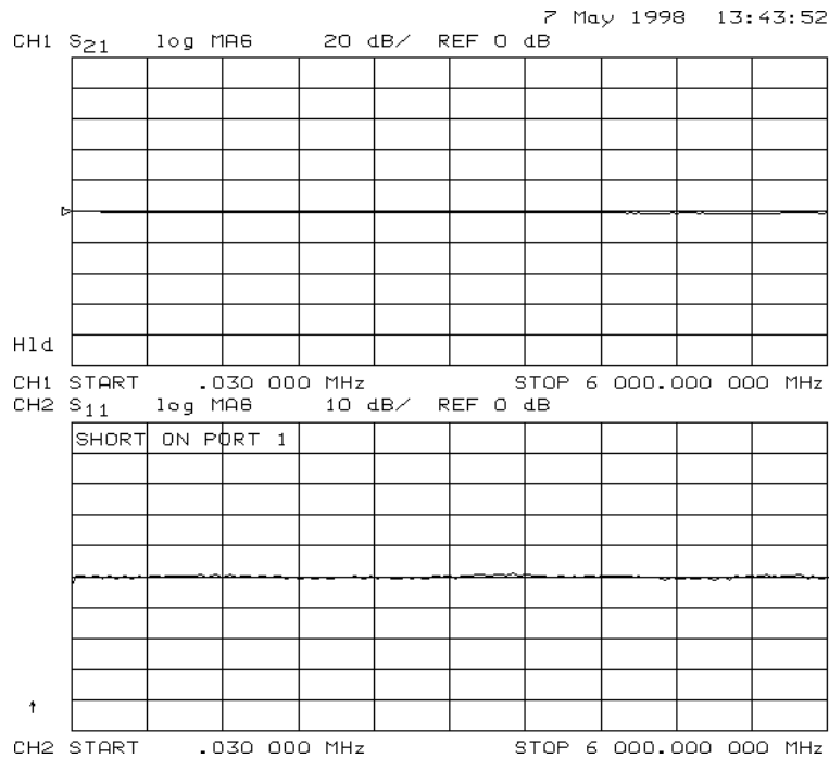
Figure 4-13 Example of a Good Measurement
