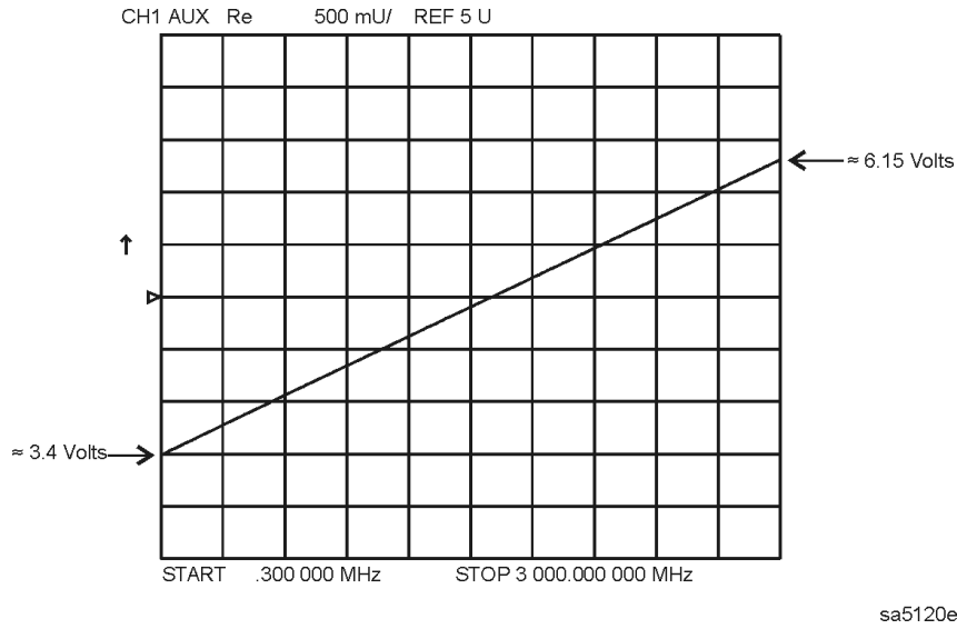
Figure 4-6 ABUS Node 16: 1 V/GHz
