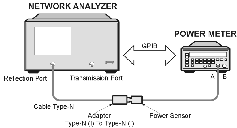
Figure 2-69 Power Meter Calibration Setup
