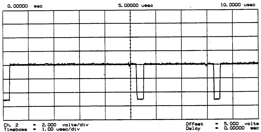
Figure 7-15 L ENREF Line at A12P2-16 (Preset)
