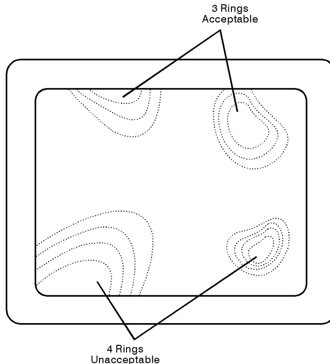
Figure 6-5 Newtons Rings
