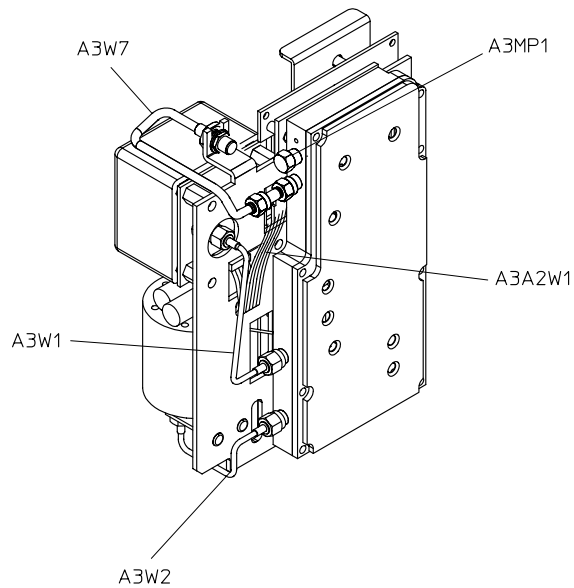
Figure 13-16 8753ET: Cables, Source
