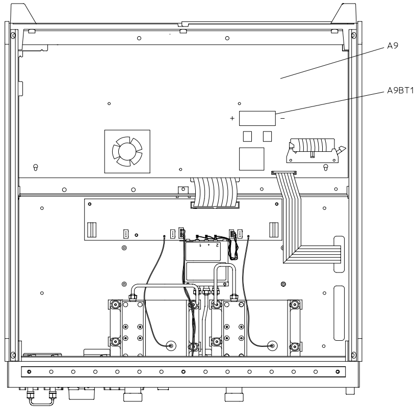
Figure 14-12 A9BT1 Battery
